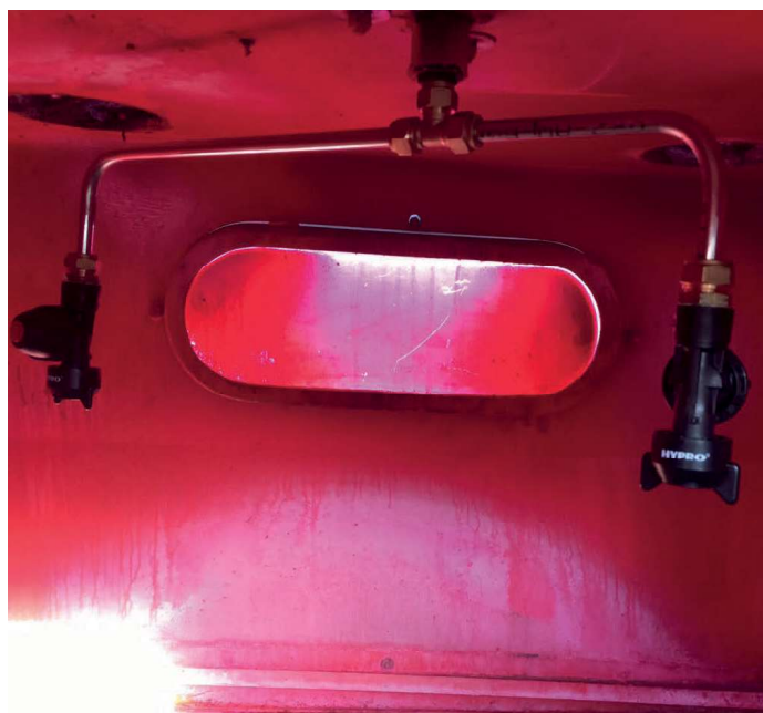
Figure 4. Top: roller table in operation. Bottom: rotating twin nozzles under the hood
