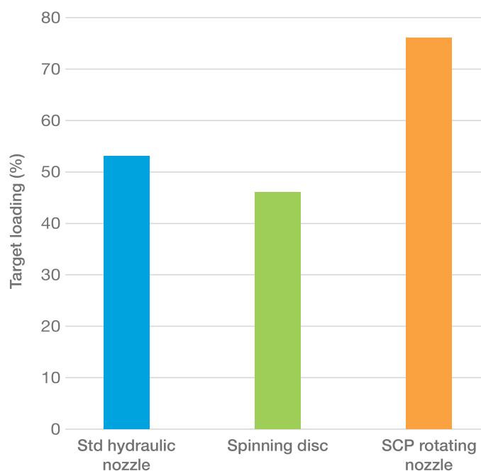
Figure 3. Efficacy of application by different nozzle types, Syngenta & Team Sprayers
